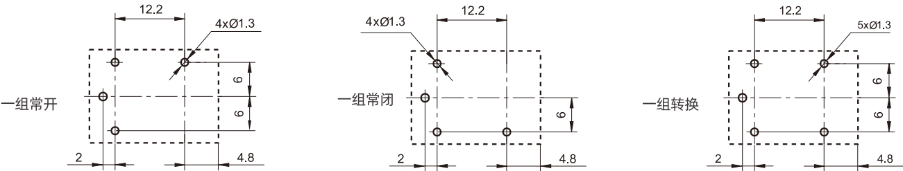
接线图(底视图) Wiring diagram (bottom view)
