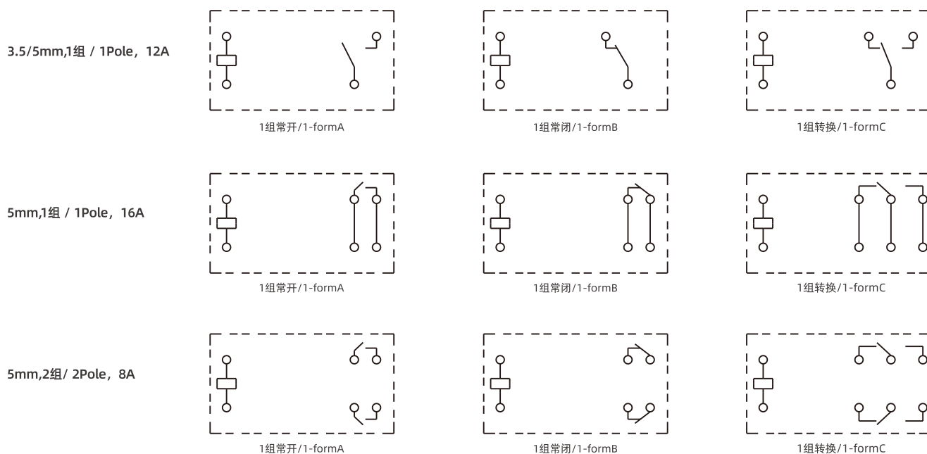
接线图(底视图) Wiring diagram (bottom view)
