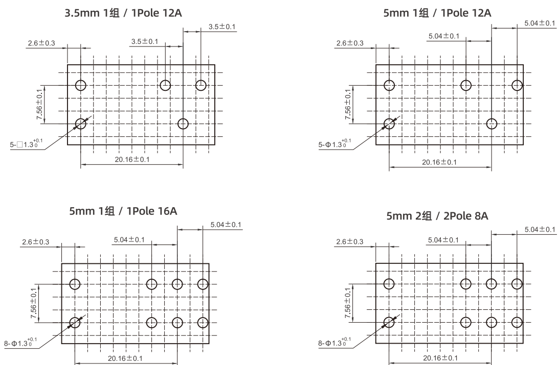
安装孔尺寸(底视图) Mounting hole size (bottom view)
