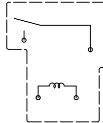
接线图 (底视图) Wiring diagram (bottom view)
