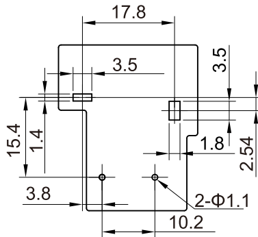
安装孔尺寸 (底视图) Mounting hole size (bottom view)
