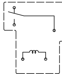
接线图 (底视图) Wiring diagram (bottom view)
